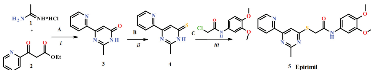
Scheme 1. Reagents and conditions: (i) MeONa/ dry MeOH, 80 °C; (ii) Toluene, RL, t°; (iii) Et 3 N, dry DMF, 60 °C.
