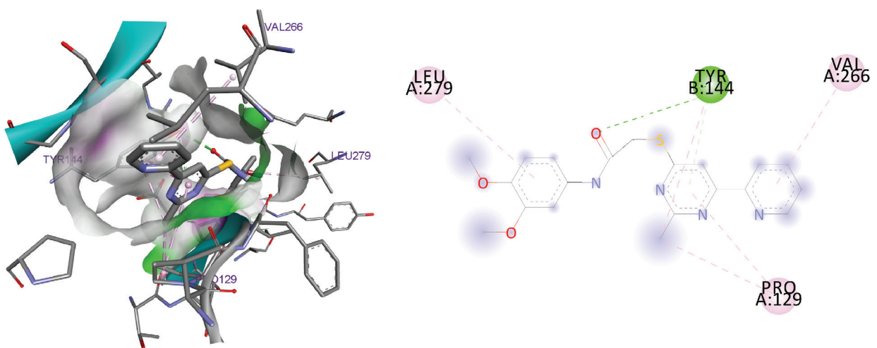
Figure 6. 3D and 2D interaction between NMDAR and Epirimil ligand.
