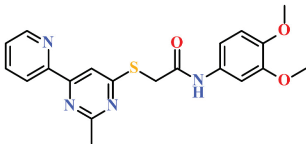
Figure 1. N-(3,4-dimethoxyphenyl)-2-((2-methyl-6-(pyridin-2-yl)pyrimidin-4-yl)thio)acetamide (Epirimil).
