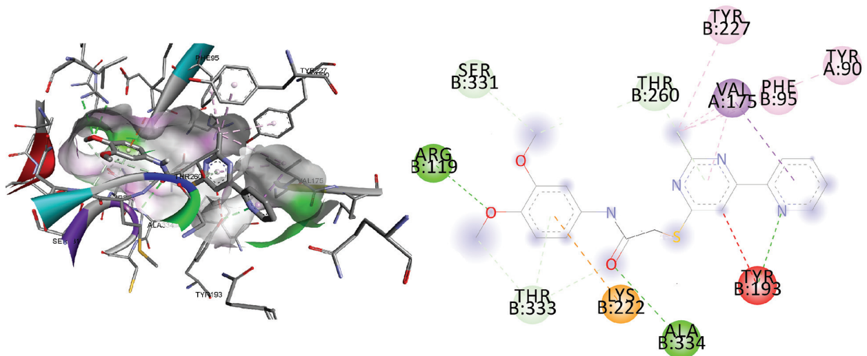
Figure 4. 3D and 2D interaction between hBCATc and Epirimil ligand.
