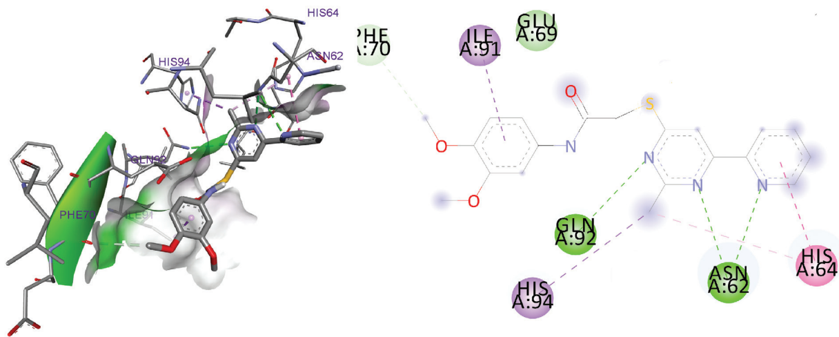
Figure 5. 3D and 2D interaction between CAII and Epirimil ligand.
